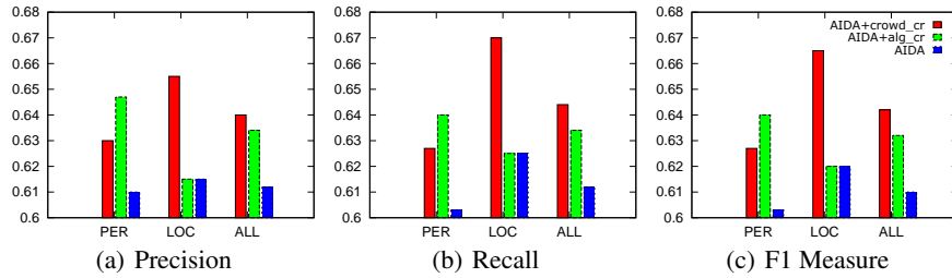
Fig. 5. NED Performance Comparison
