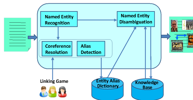
Fig. 1. Framework for NERD, CR, and AD.
