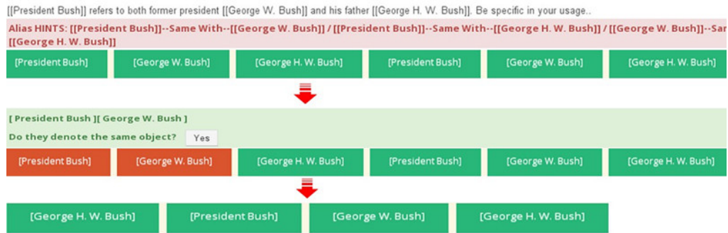
Fig. 2. Linking-Game Interface
